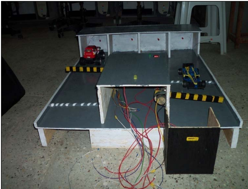
Fig-3: 2G Parking System
